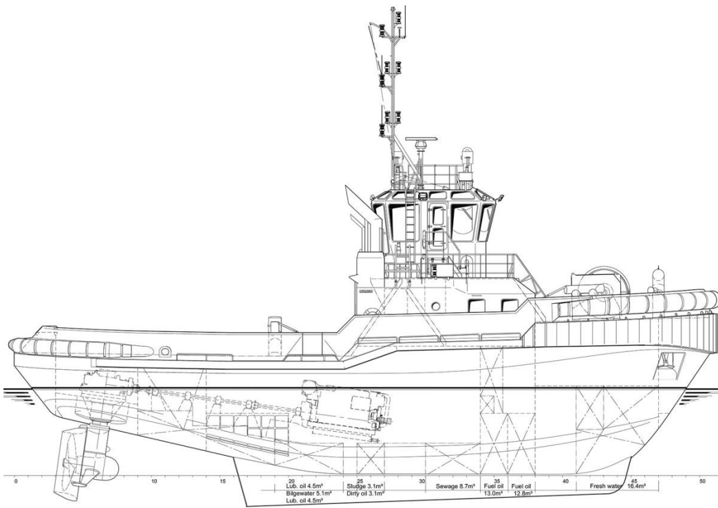
SIDE VIEW
